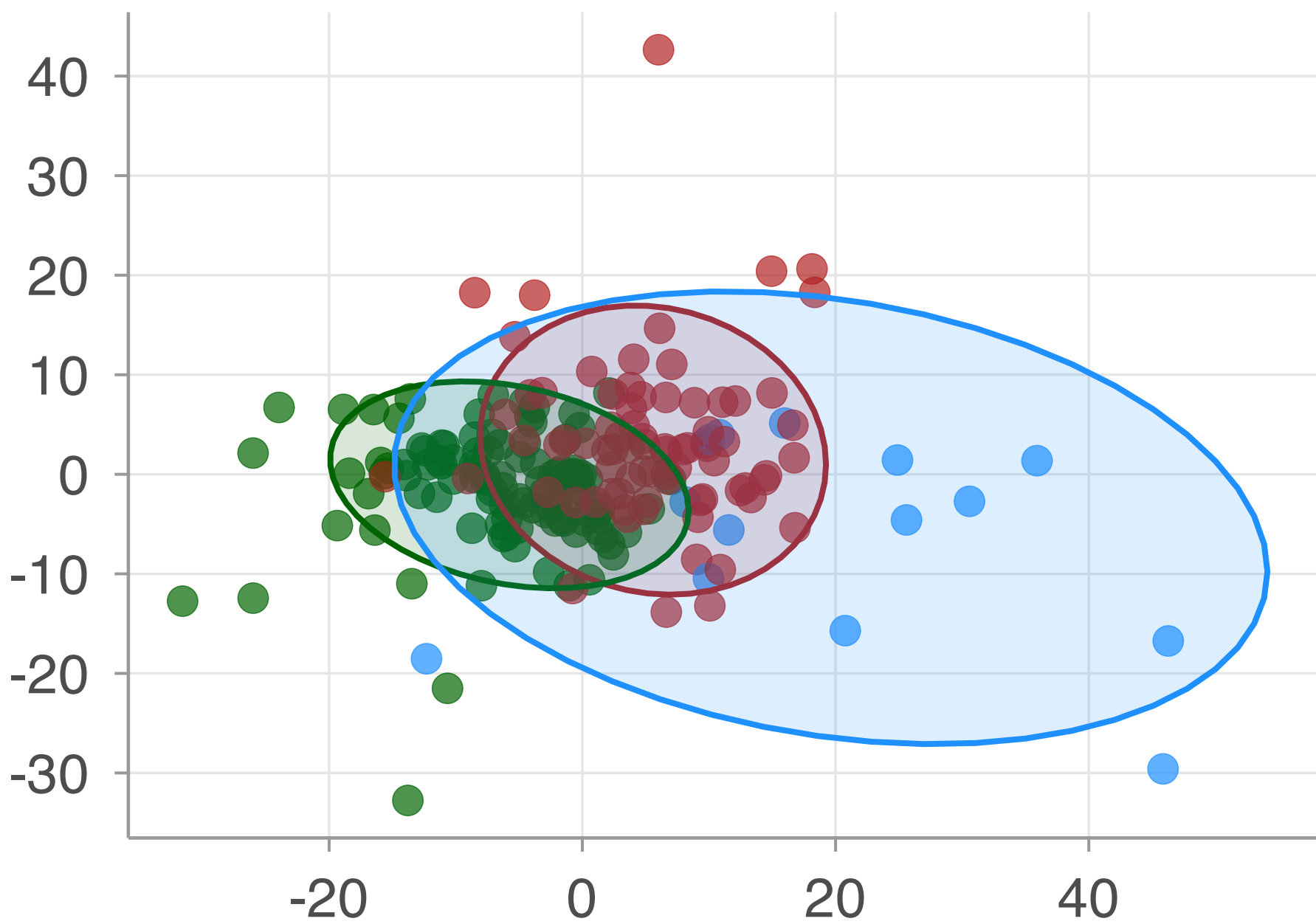
PC2 (20.93% variance)
