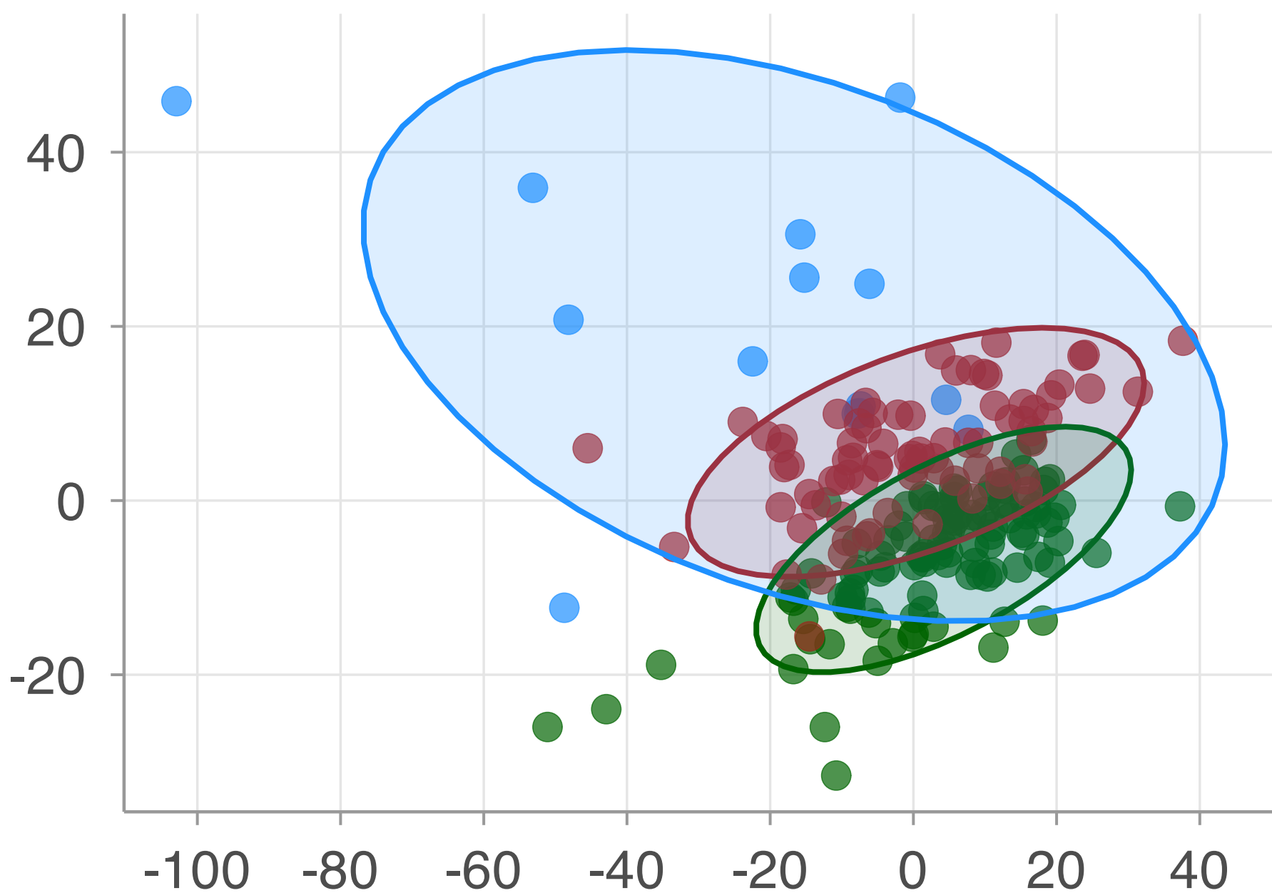
PC1 (47.46% variance)
